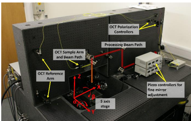
Figure 1. Set-up for OCT integrated with laser processing.
