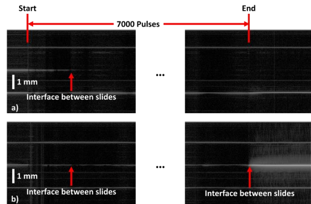
Figure 5: OCT M-modes of a) weld crossing the interface between gaps and b) not crossing the interface. Due to the long length of exposure, the middle of the images have been removed for brevity.
