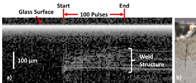
Figure 3: a) OCT monitoring of weld structure formation in bulk \text{SiO}_2 and b) corresponding microscope image of structure. The depth scale is the same for both images.
