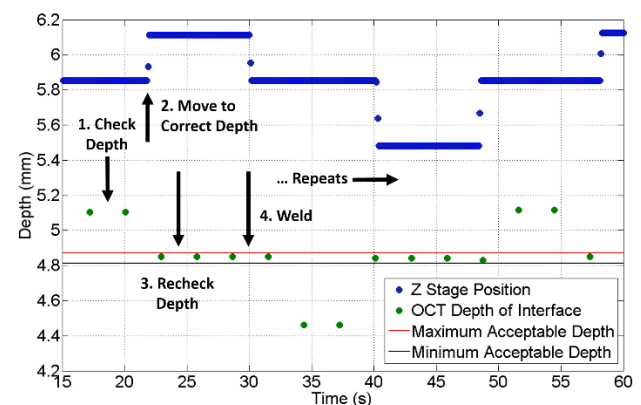
Figure 2. In-situ depth control data for OCT Welding.
