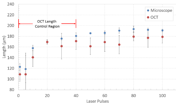
Figure 4: Length of weld structure as measured by OCT and optical microscopy as a function of laser pulses in bulk \text{SiO}_2 .
