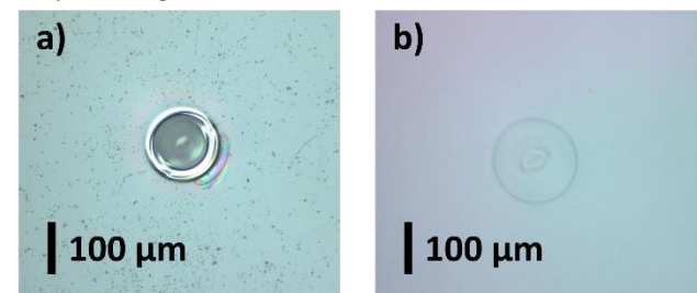
Figure 6: Top down optical microscope image of a) weld crossing the interface between gaps and b) not crossing the interface.
