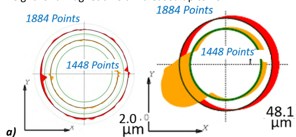
Figure 2: Deviation plot of the sphere: a) at 0mT; b) at 3mT
