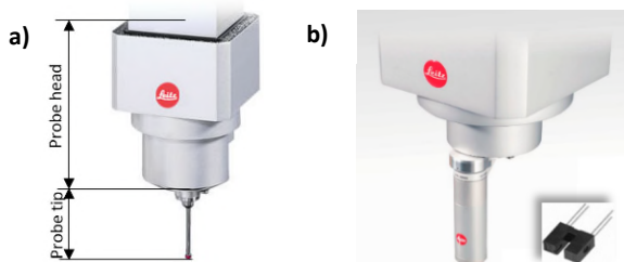
Figure 1: a) The probing parts b) The Precitec LR sensor and the SHARP optical switch
