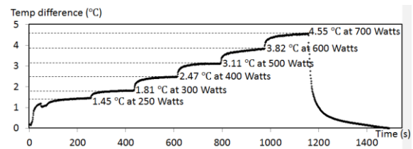
Fig. 7: TD of the coolants through ICP torch
